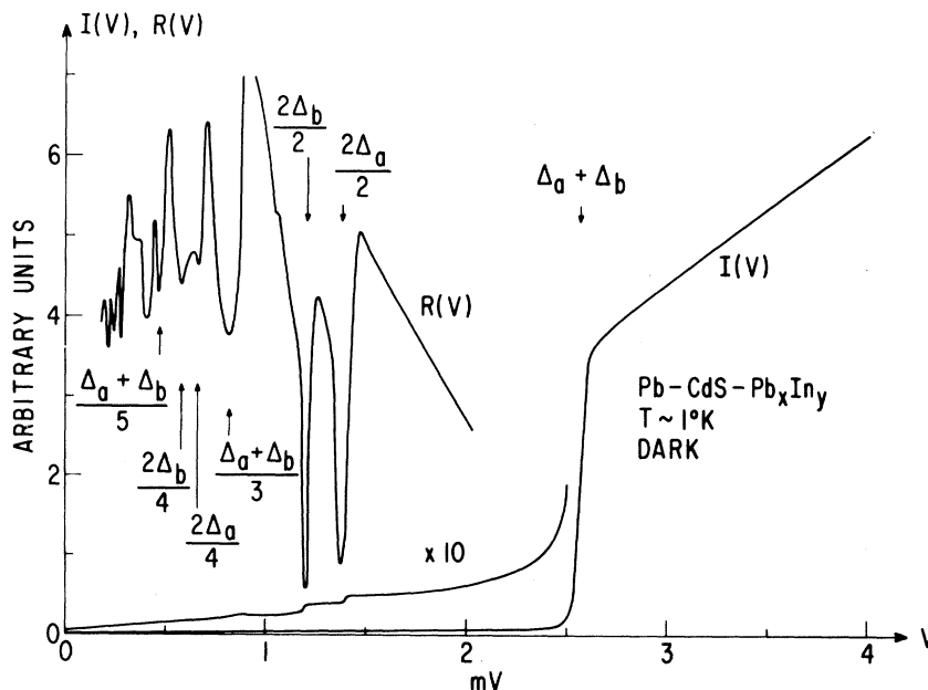
FIG. 14. Current-voltage and dynamic resistance characteristics of a Pb-CdS-Pb x In y junction. Because the gaps are approximately equal, the two even series and the single odd series can be identified. a refers to Pb and b to Pb x In y . Again, at lower voltages it becomes difficult to distinguish between the series themselves and small Fiske steps.
